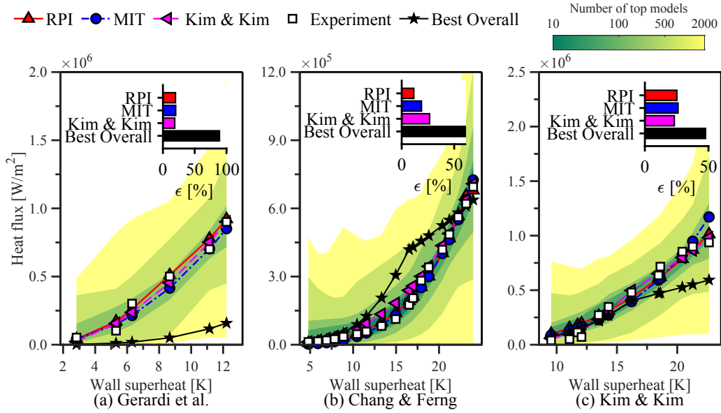
Figure 14: Sample boiling curves for pool boiling datasets.
