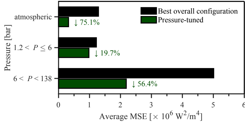
Figure 9: Comparison of prediction errors between the best overall configuration and pressure-tuned configurations.
