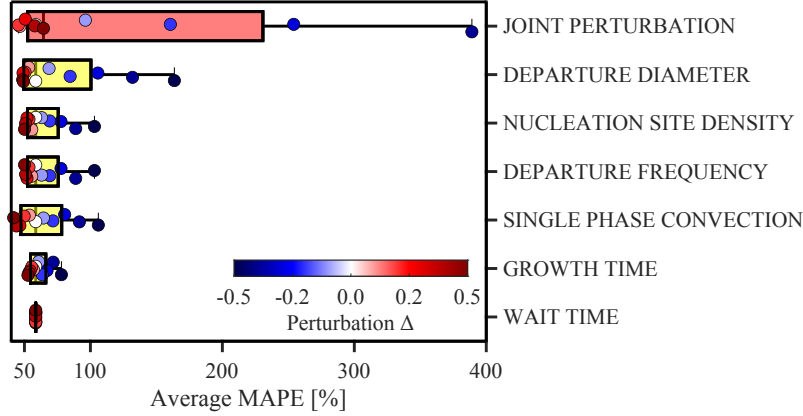
Figure 11: Sensitivity of bubble dynamic parameters evaluated by perturbing each parameter across a range of \pm 50\% around their nominal value, while keeping the rest fixed. For each perturbation, the mean MAPE was computed across all cases. Box plots summarise the spread of average MAPE values for each sub-model category. Overlaid scatter points show individual perturbation results, coloured according to perturbation level.
