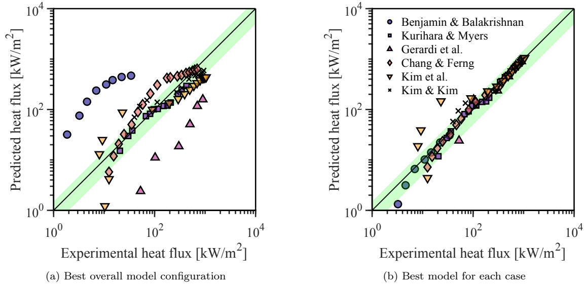
Figure 13: Comparison between the best overall configuration and per-case best configuration in predicting heat flux in pool boiling. The green band represents \pm 50\% deviations.
