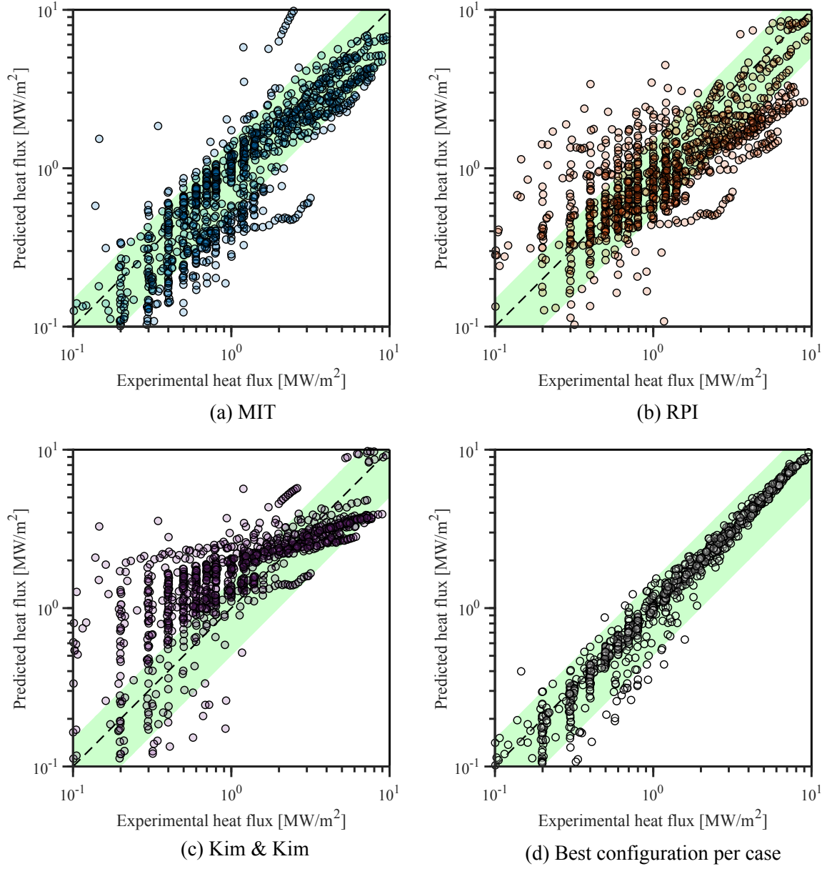
Figure 7: Predicted vs. experimental heat fluxes for the three heat flux partitioning models. Shaded green region illustrates predictions within \pm 50\% of the experimental values. Subplots (a) to (c) show the configurations with the lowest global error (averaged across all datasets) for each HFP model. Subplot (d) combines all the configurations with the minimum error for each case.
