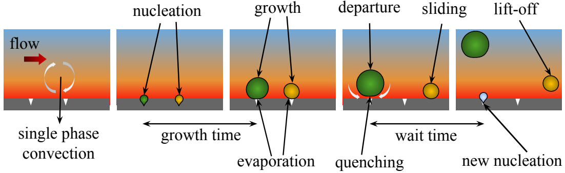
Figure 1: A simplified representation of boiling process illustrating key phenomena and bubble dynamics parameters.
