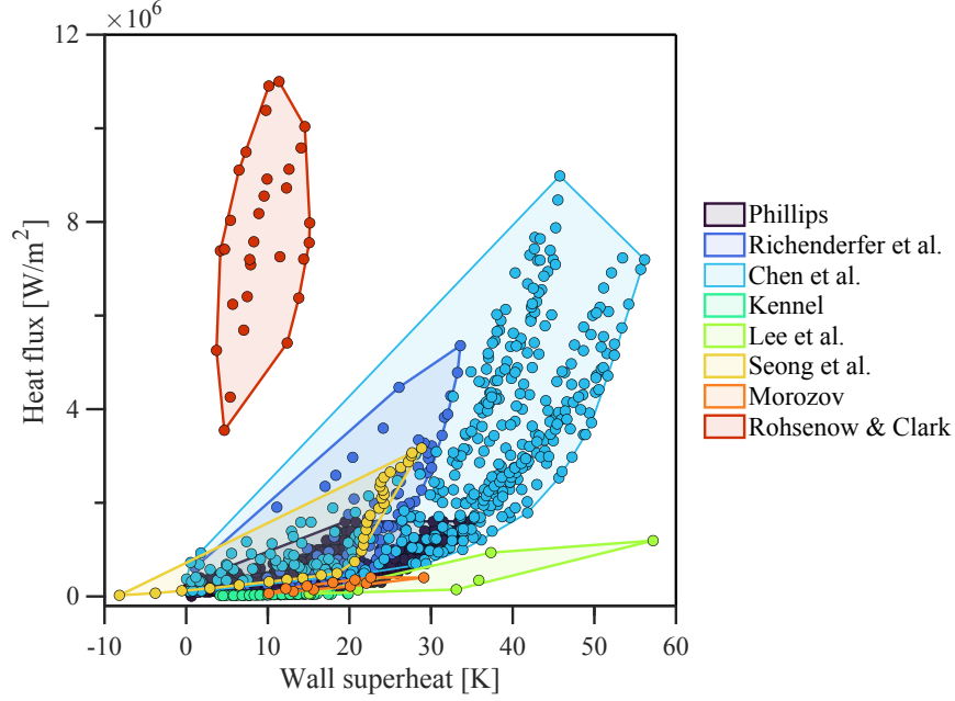
Figure 4: Boiling curves for flow boiling data selected for the assessments. Each shaded region represents a different datasets shown in Table 2.
