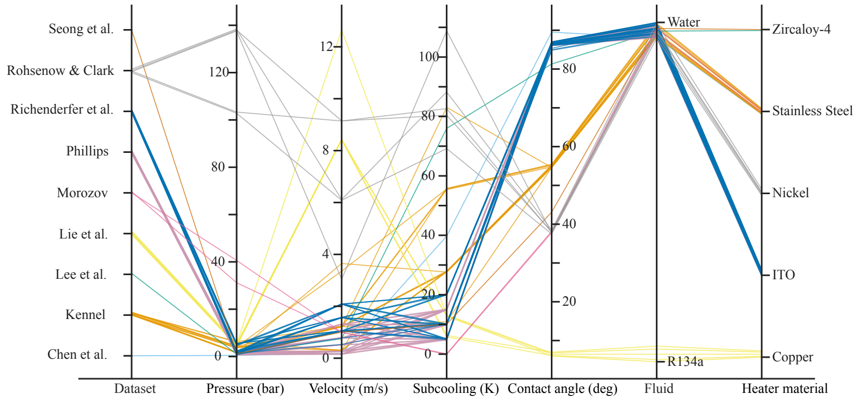
Figure 3: Flow boiling datasets in Table 2 visualised as a parallel plot illustrating the spread and variability of key parameters.
