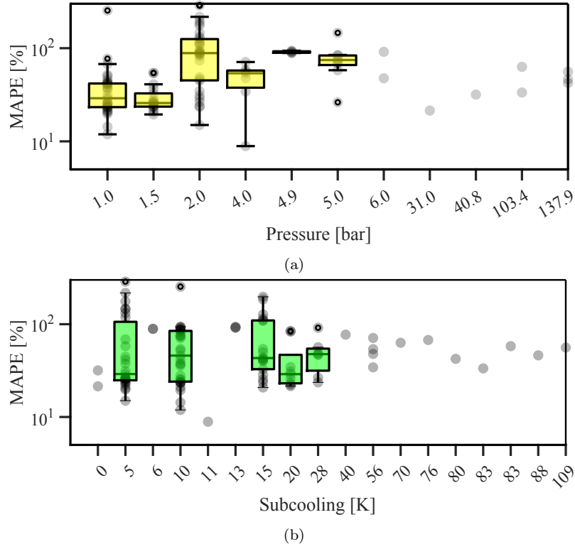
Figure 8: Mean-absolute percentage error of best-performing HFP configuration vs. pressure and subcooling.
