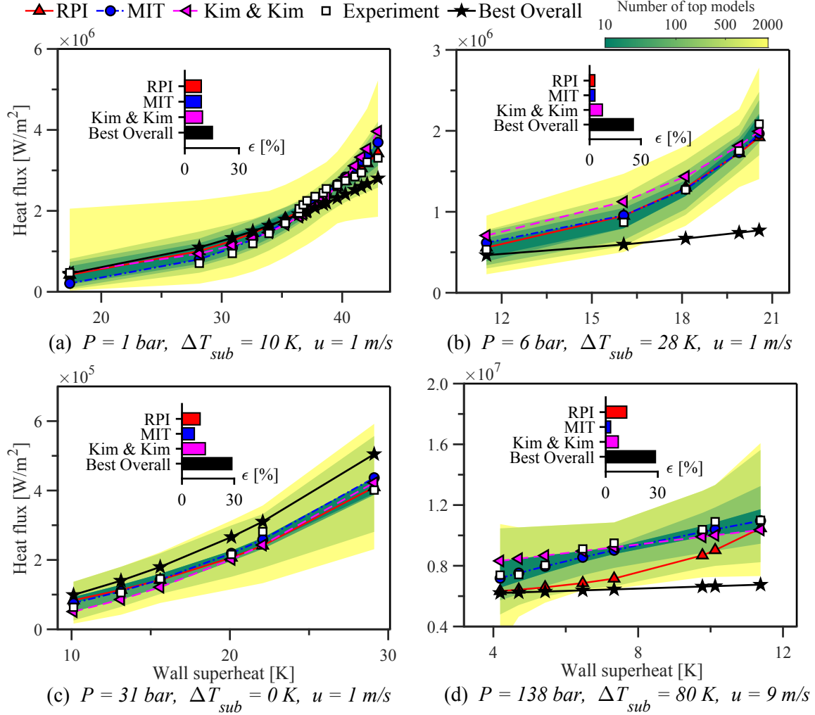
Figure 5: Sample boiling curves for different flow conditions. Shaded regions indicate the envelope formed by the minimum and maximum predictions among the top- n model configurations, ranked by agreement with experimental data. For each case, the best-performing prediction from the HFP models—RPI, MIT, and Kim & Kim—is also shown for comparison. The bar charts show the mean-absolute percentage error relative to the experimental measurements.
