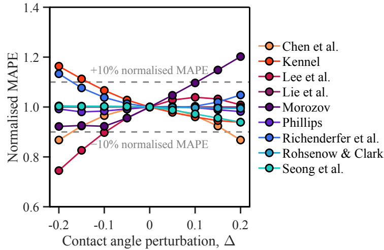
Figure 10: Sensitivity of the best overall configuration to the contact angle perturbations. Contact angle values are perturbed by \pm 20\% of the nominal values used in Table 2. The normalised MAPE represents the average mean-absolute percentage error with the perturbed contact angle divided by the average MAPE using the nominal contact angle.
