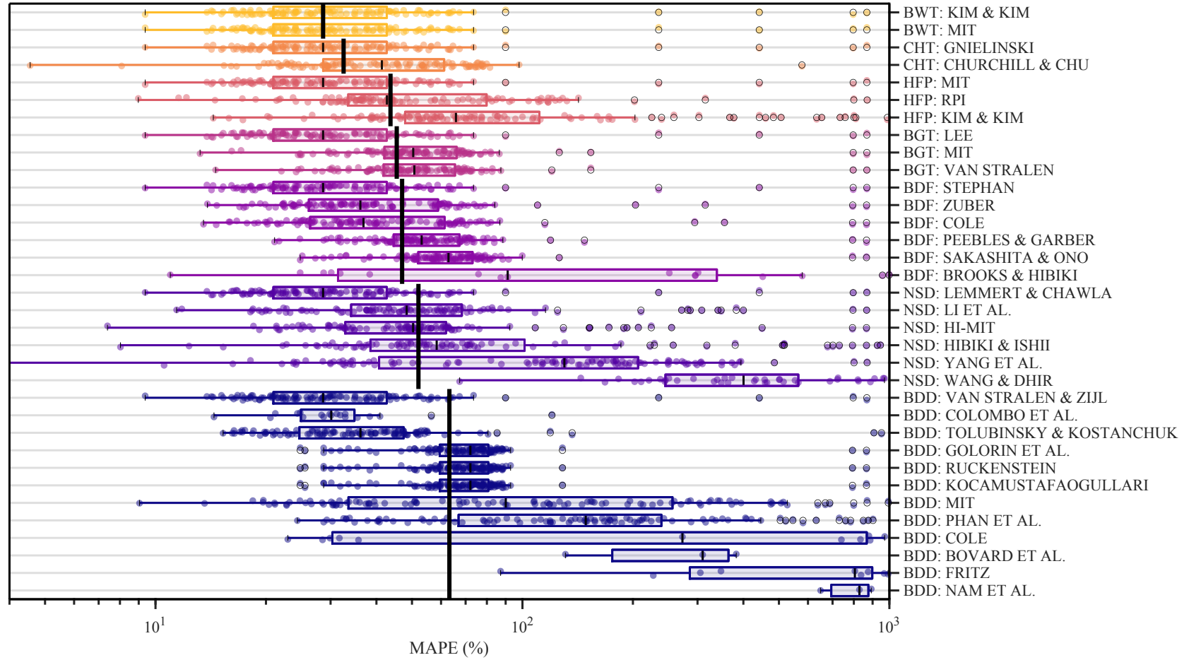
Figure 12: Sensitivity analysis of all the sub-models. Each sub-model shown corresponds to a modification of the baseline configuration (based on the best overall configuration) by replacing a single sub-model while holding all others fixed. The distribution of mean-absolute percentage error is computed per case (shown as scatter points) across all the dataset. Box plots and overlaid scatter points indicate the variation in prediction accuracy for each sub-model choice. Sub-models are grouped and colour-coded by category. Solid black lines indicate the median MAPE across all sub-models within each category.
