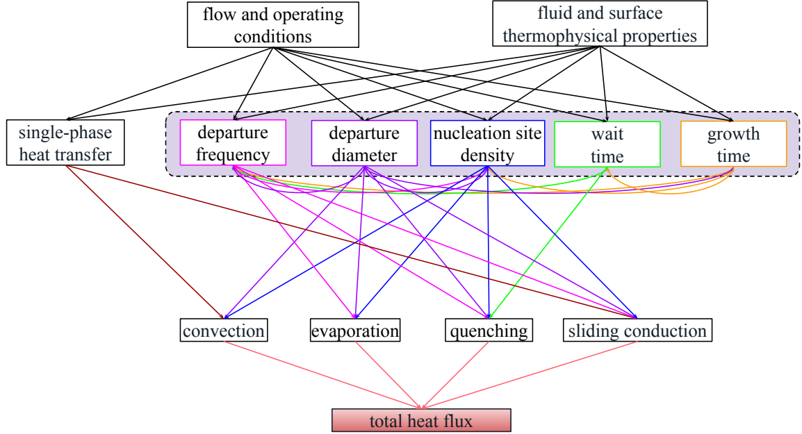
Figure 2: Various components and their interdependencies in heat flux partitioning modelling.
