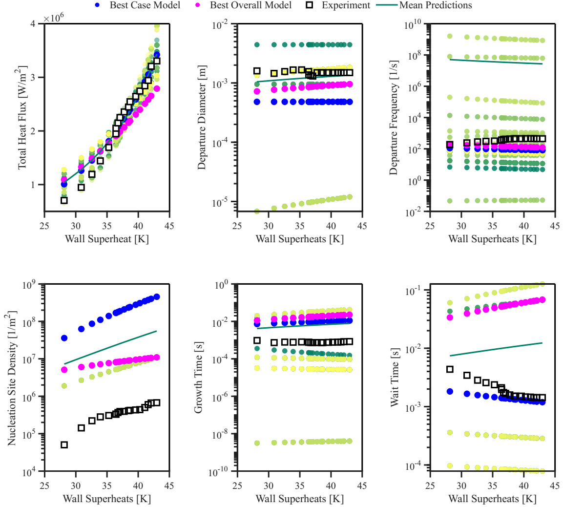
Figure 6: Comparison of the predicted and experimental total heat flux and individual bubble parameters for Richenderfer et al. [18] at p = 1.01 bar, u = 1.04 m/s, and \Delta T_{\text{sub}} = 10.0 K. The top 200 models are shown as green scatters.
